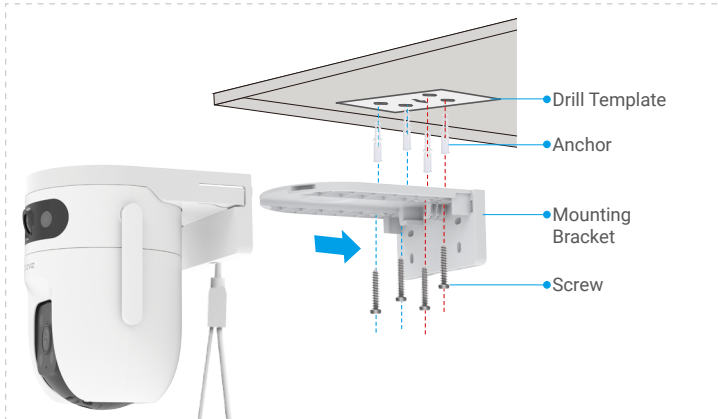
Fig. 1 Ceiling Mount
