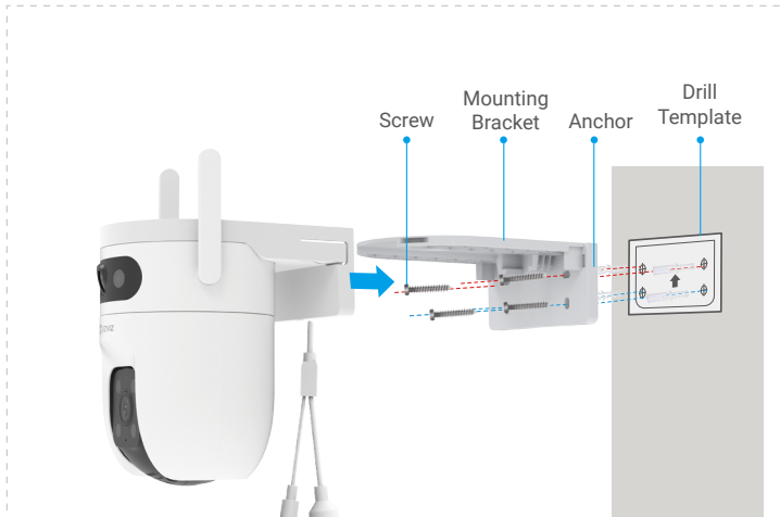
Fig. 2 Wall Mount
